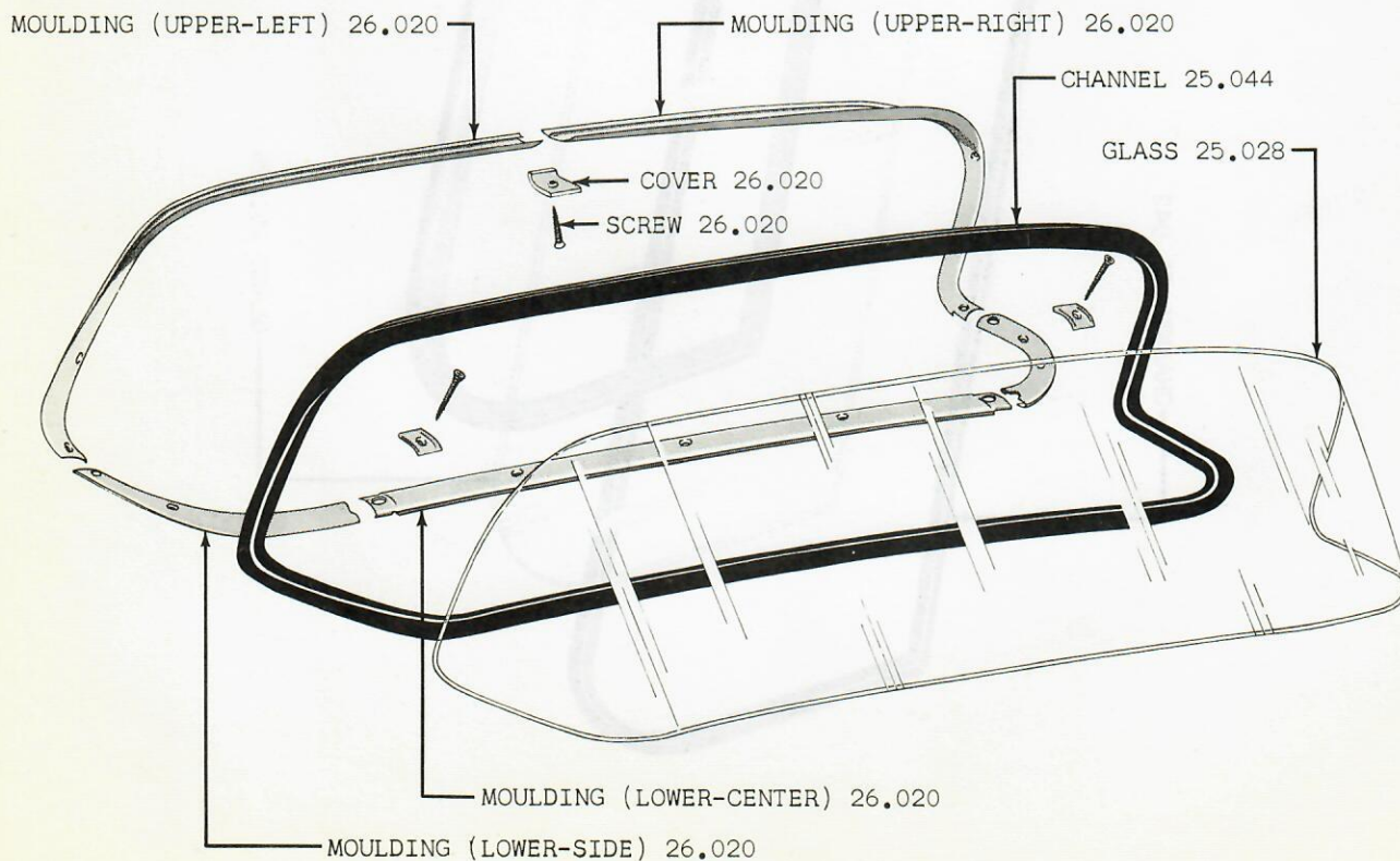
GROUP 25 - FIG. 5 - REAR WINDOW GLASS, CHANNEL AND FINISH MOULDINGS 10-20-80 SEDAN
